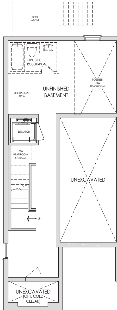
BASEMENT PLAN
