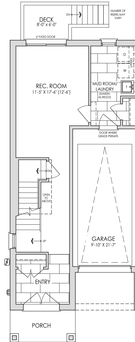
GROUND FLOOR 651 SQ FT
