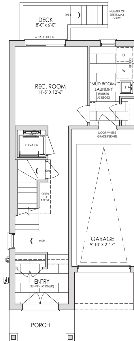
GROUND FLOOR WITH ELEVATOR 651 SQ FT
