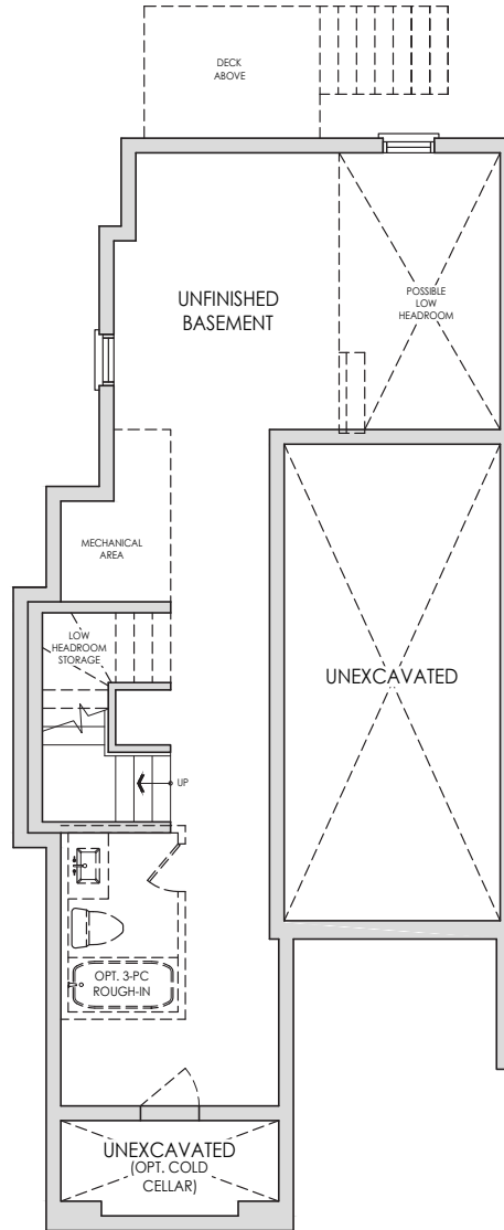
BASEMENT PLAN
