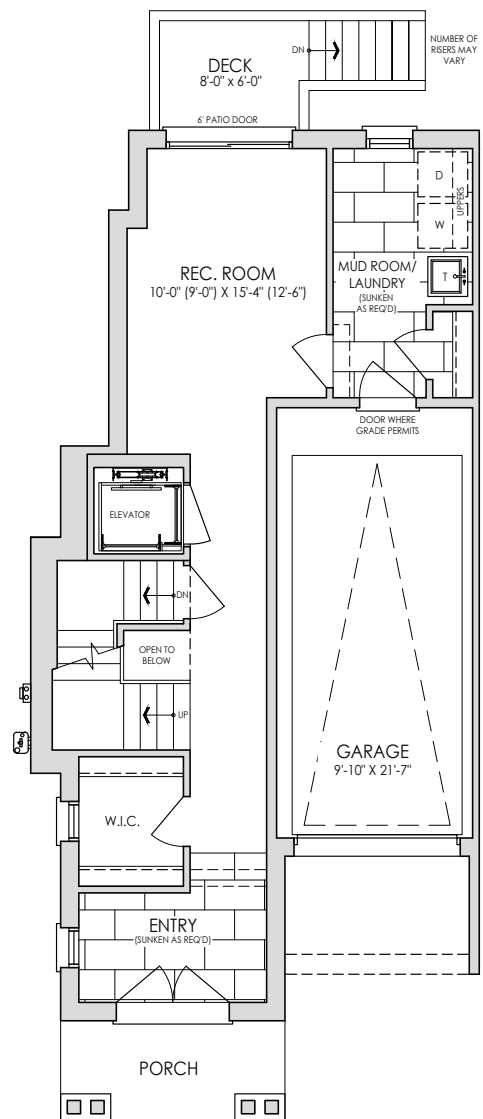
GROUND FLOOR WITH ELEVATOR 651 SQ FT
