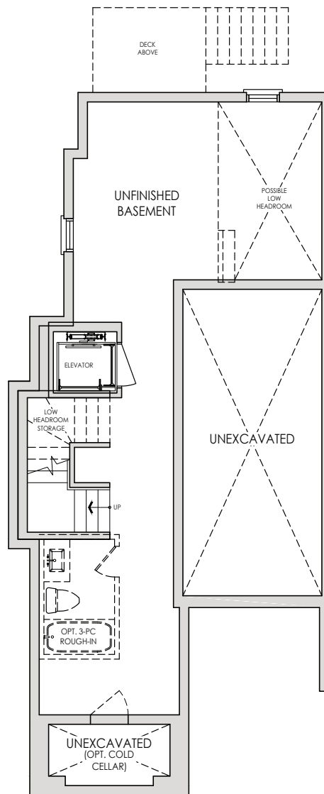
BASEMENT PLAN
