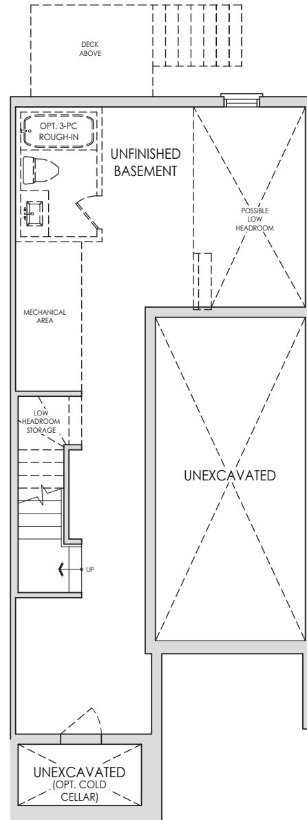
BASEMENT PLAN
