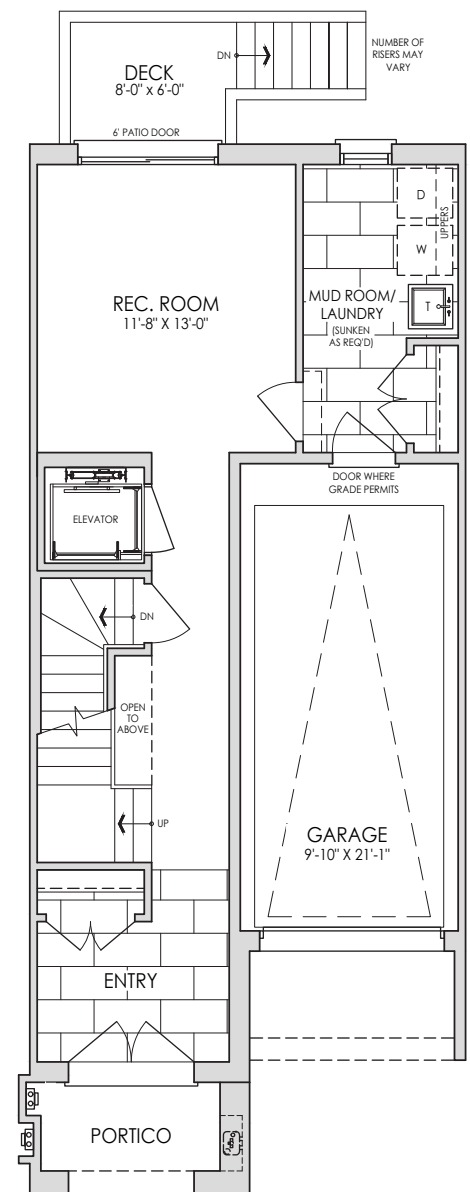
GROUND FLOOR WITH ELEVATOR 551 SQ FT
