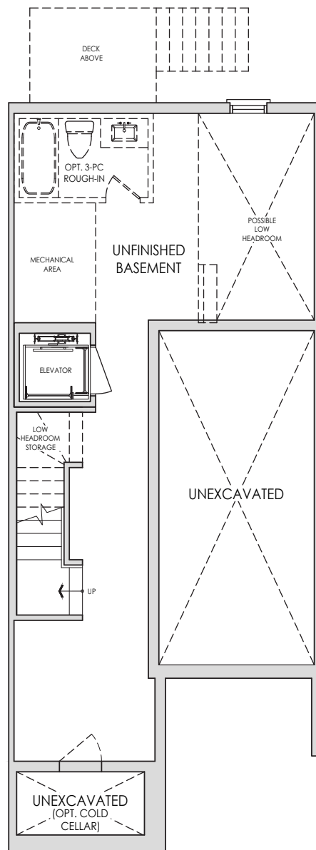
BASEMENT PLAN
