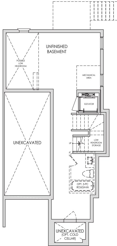
BASEMENT PLAN
