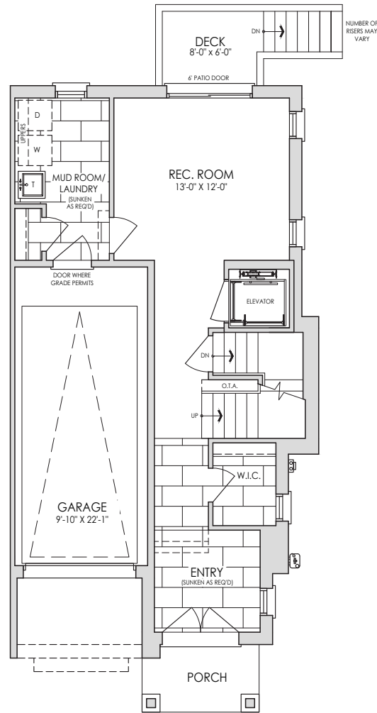
GROUND FLOOR WITH ELEVATOR 603 SQ FT
