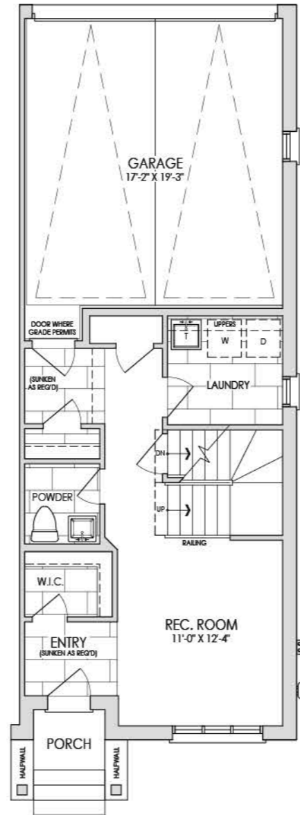
GROUND FLOOR 509 SQ. FT.
