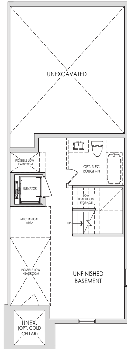
BASEMENT PLAN
