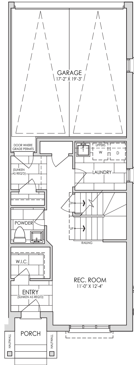
GROUND FLOOR 508 SQ FT
