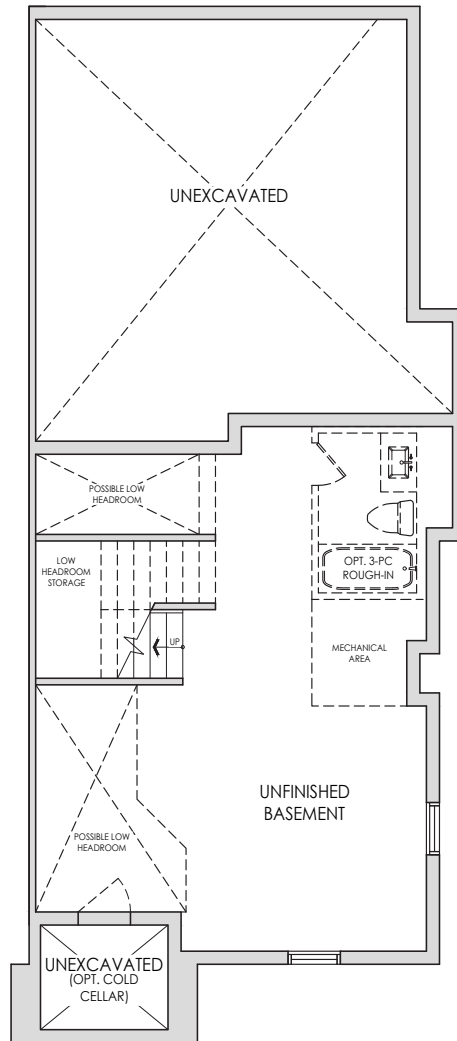
BASEMENT PLAN
